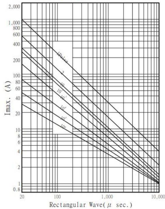
Pulse Life time Ratings-14mm 14N 180M~14N 680K
