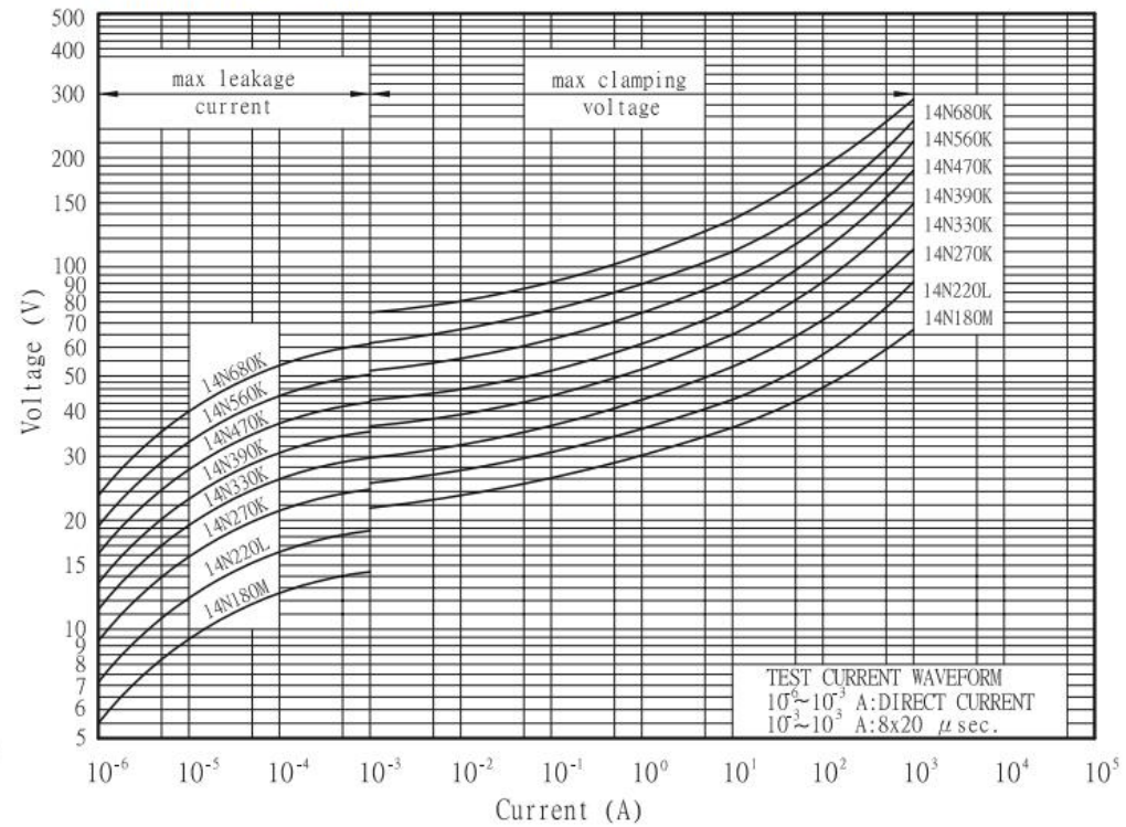
V-I Characteristic Curve-14mm 14N 180M~14N 680K
